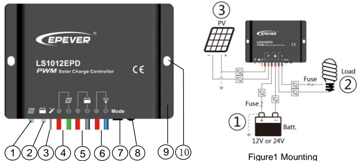
Figure1 Mounting
